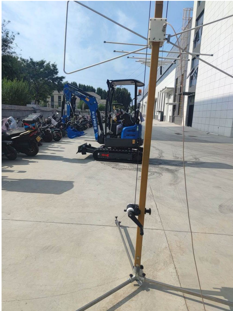
Photograph 1: Set-up for radiated electromagnetic disturbances above 30MHz
