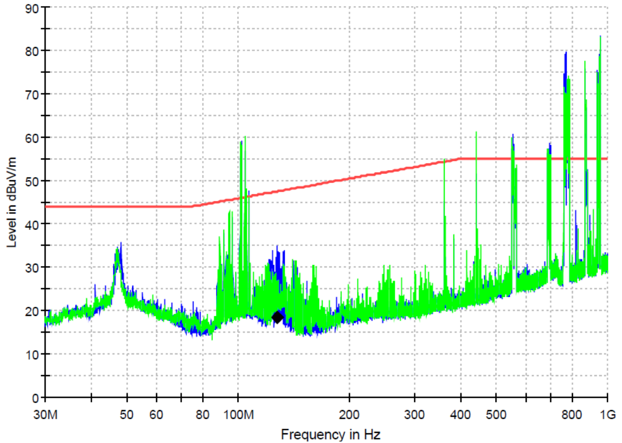
Figure 8: Spectral diagrams and measurement results for 30-1000MHz, Vertical polarization, P1, R10 (with KD192F)
