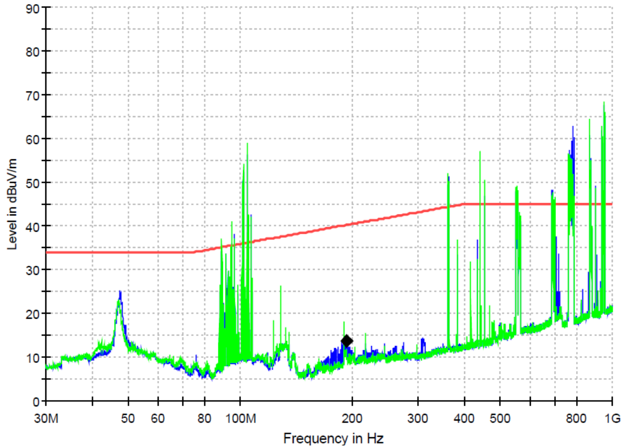
Figure 16: Spectral diagrams and measurement results for 30-1000MHz, Vertical polarization, P2, R10 (with Z482-EF04_CN4)
