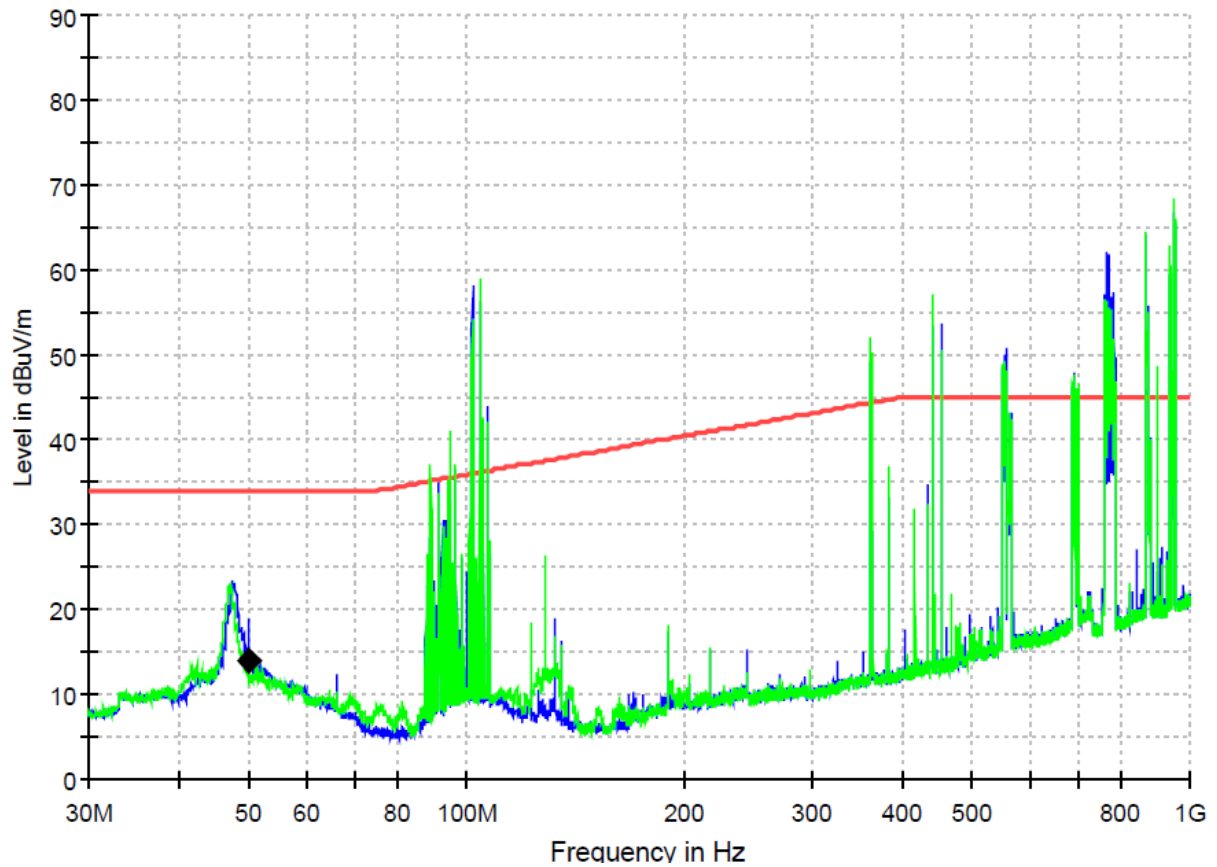
Figure 18: Spectral diagrams and measurement results for 30-1000MHz, Vertical polarization, P1, R10 (with KD192F)
