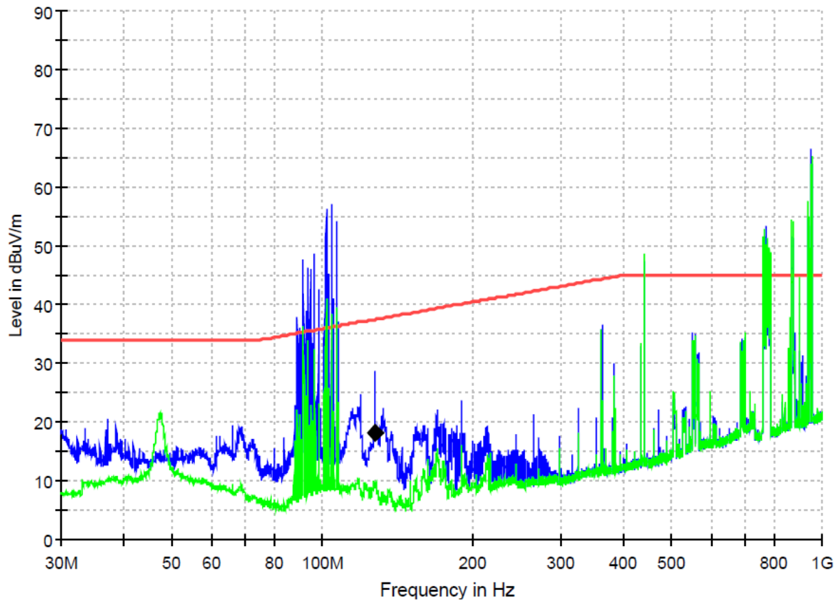
Figure 15: Spectral diagrams and measurement results for 30-1000MHz, Horizontal polarization, P2, R10 (with Z482-EF04_CN4)
