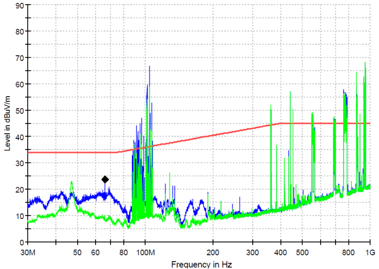
Figure 20: Spectral diagrams and measurement results for 30-1000MHz, Vertical polarization, P2, R10 (with KD192F)
