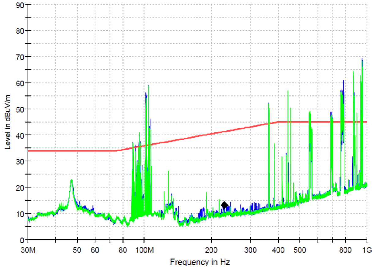
Figure 14: Spectral diagrams and measurement results for 30-1000MHz, Vertical polarization, P1, R10 (with Z482-EF04_CN4)
