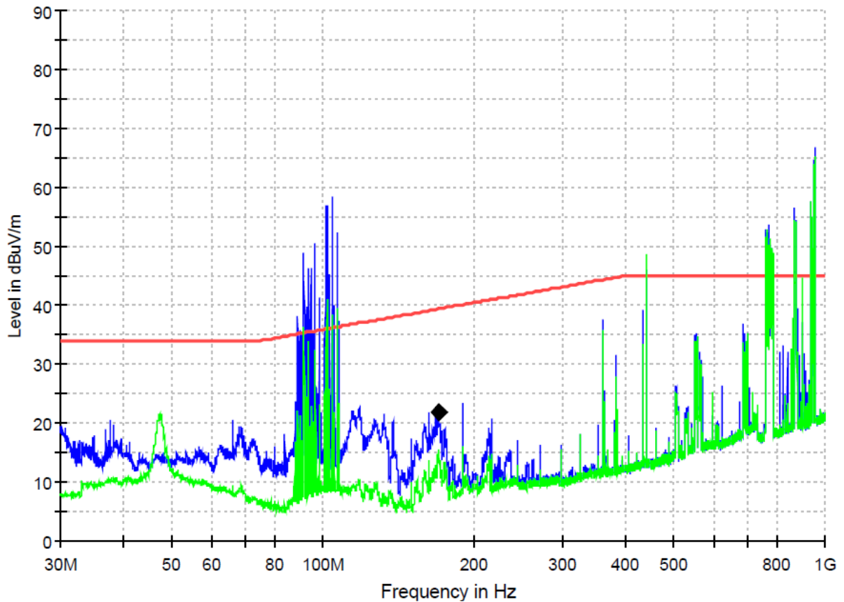
Figure 13: Spectral diagrams and measurement results for 30-1000MHz, Horizontal polarization, P1, R10 (with Z482-EF04_CN4)
