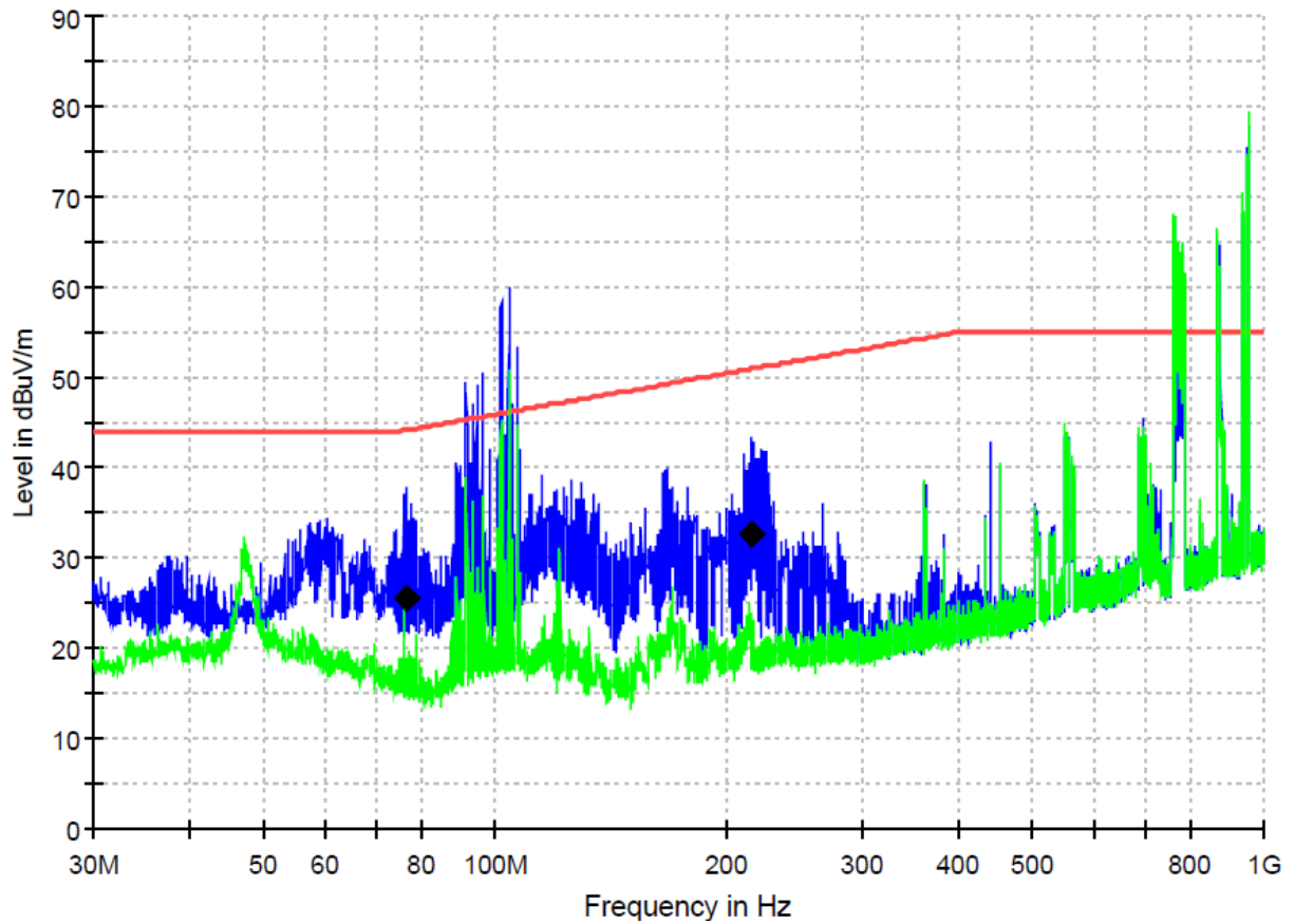
Figure 3: Spectral diagrams and measurement results for 30-1000MHz, Horizontal polarization, P1, R10 (with Z482-EF04_CN4)
