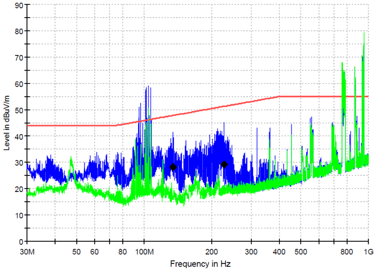
Figure 5: Spectral diagrams and measurement results for 30-1000MHz, Horizontal polarization, P2, R10 (with Z482-EF04_CN4)
