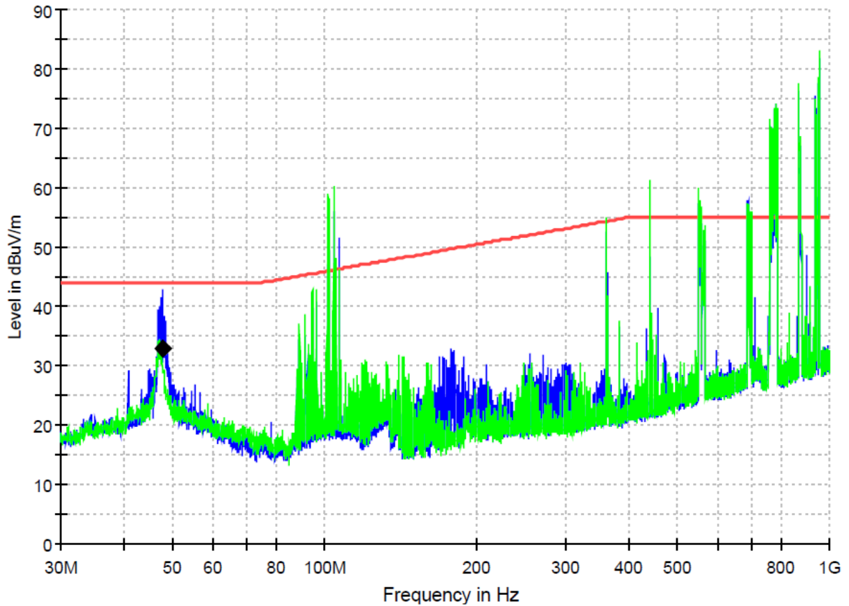
Figure 6: Spectral diagrams and measurement results for 30-1000MHz, Vertical polarization, P2, R10 (with Z482-EF04_CN4)
