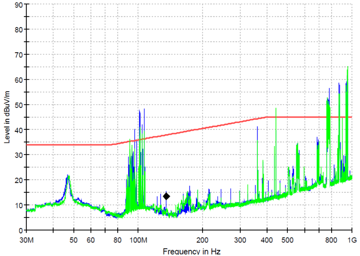
Figure 17: Spectral diagrams and measurement results for 30-1000MHz, Horizontal polarization, P1, R10 (with KD192F)
