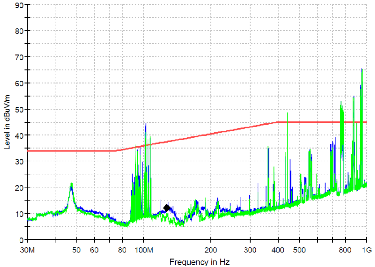
Figure 19: Spectral diagrams and measurement results for 30-1000MHz, Horizontal polarization, P2, R10 (with KD192F)
