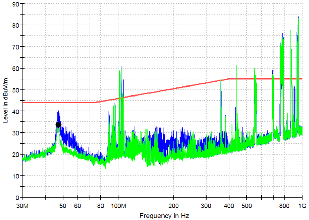
Figure 4: Spectral diagrams and measurement results for 30-1000MHz, Vertical polarization, P1, R10 (with Z482-EF04_CN4)
