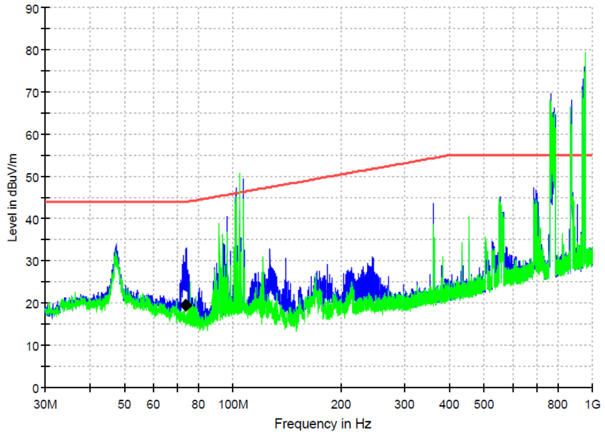
Figure 9: Spectral diagrams and measurement results for 30-1000MHz, Horizontal polarization, P2, R10 (with KF192F)
