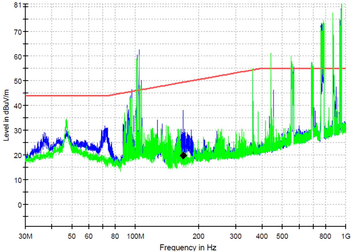
Figure 10: Spectral diagrams and measurement results for 30-1000MHz, Vertical polarization, P2, R10 (with KD192F)
