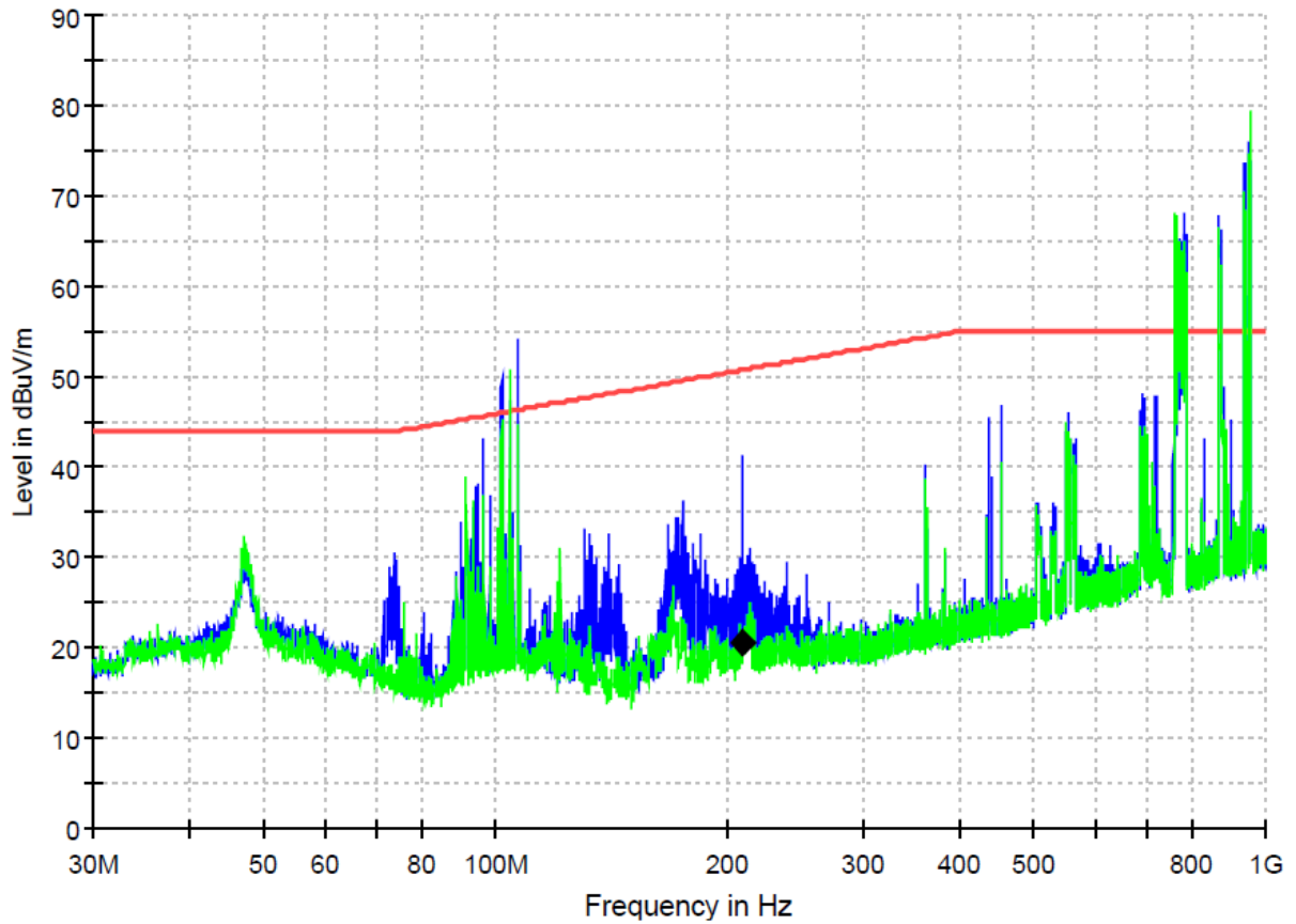
Figure 7: Spectral diagrams and measurement results for 30-1000MHz, Horizontal polarization, P1, R10 (with KD192F)
